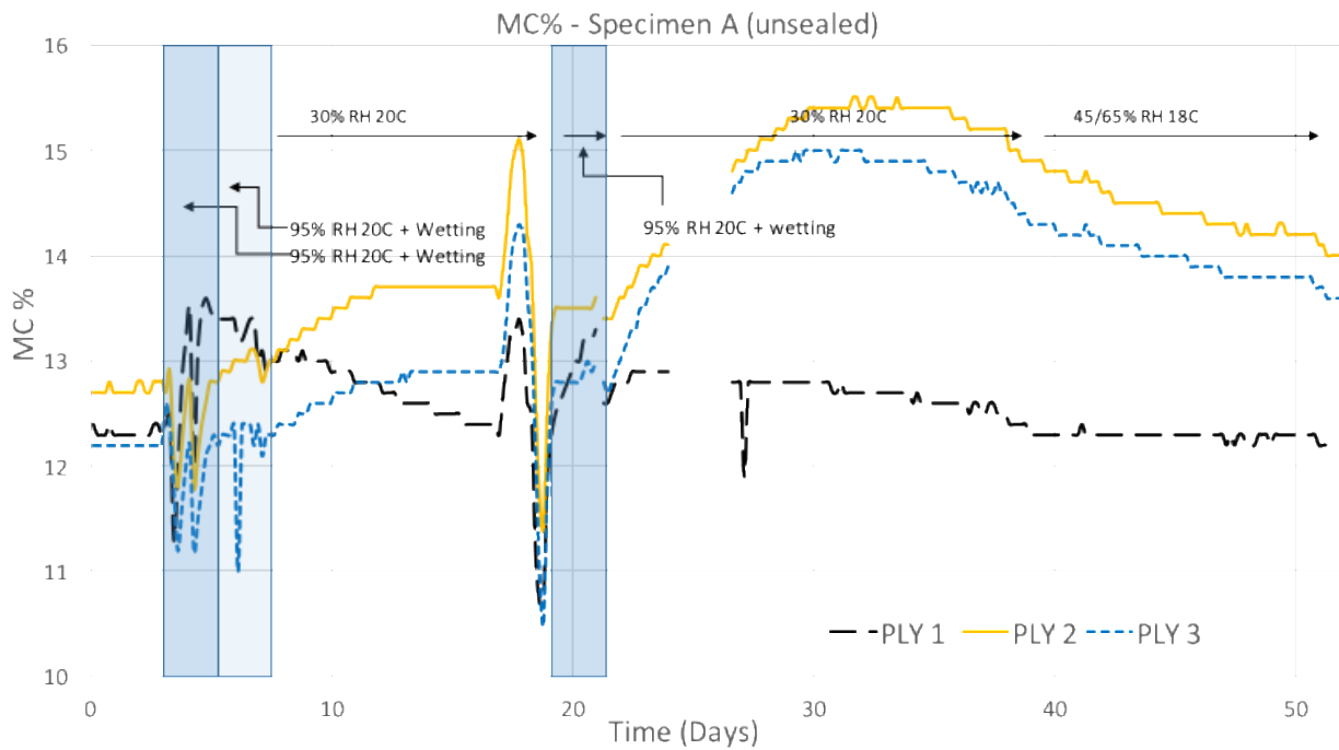
Figure 2: Moisture curves in the bottom-most ply (PLY 1), and the two plies above it (PLY 2 and PLY 3, respectively) of specimen A- unsealed over the duration of 52 days. Note: values that deviate from 20°C are not temperature-corrected; anomalous spikes in MC can be directly correlated to temperature spikes in fig. 1.
