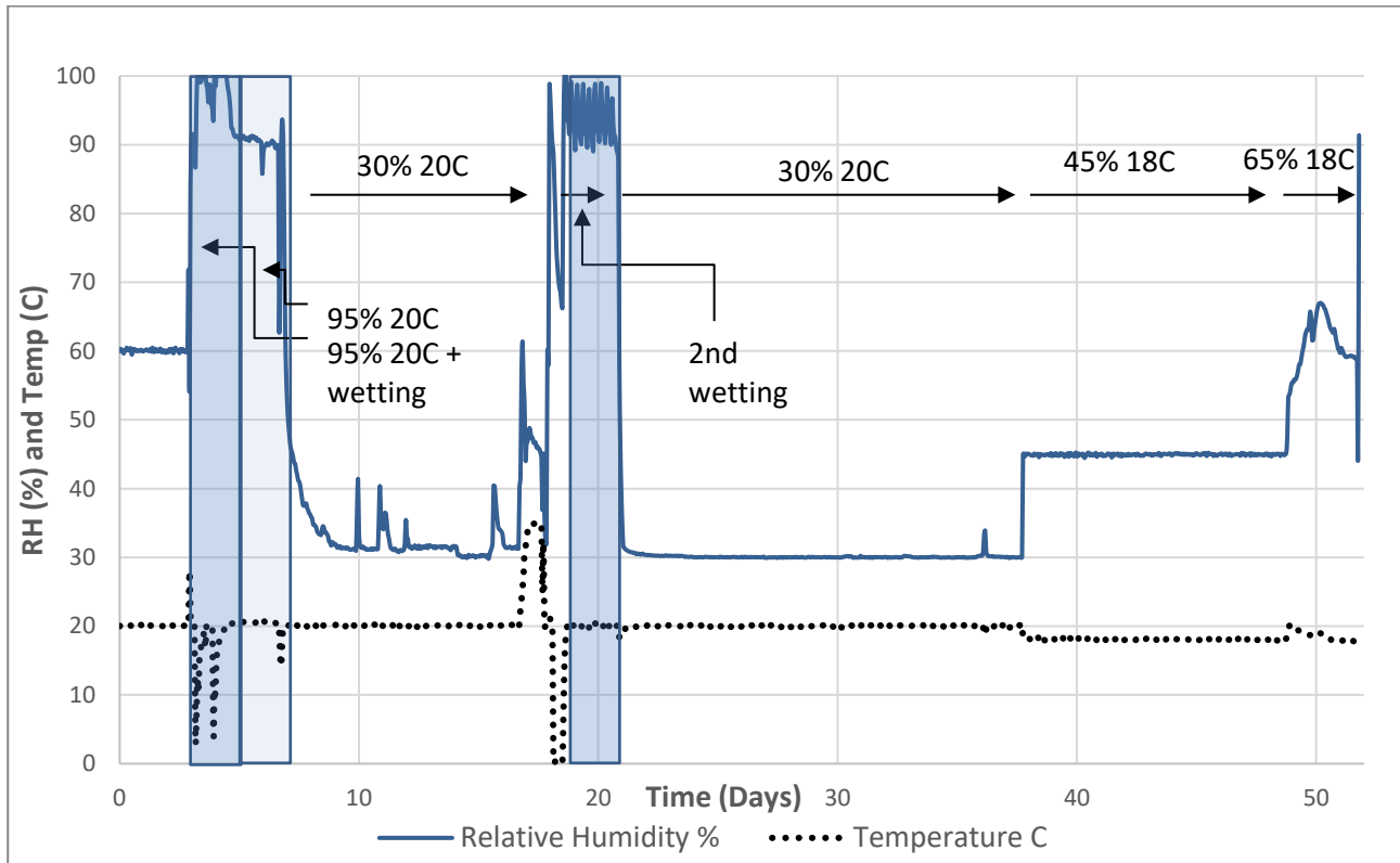
Figure 1: Climate conditions over the course of the 52-day experiment
