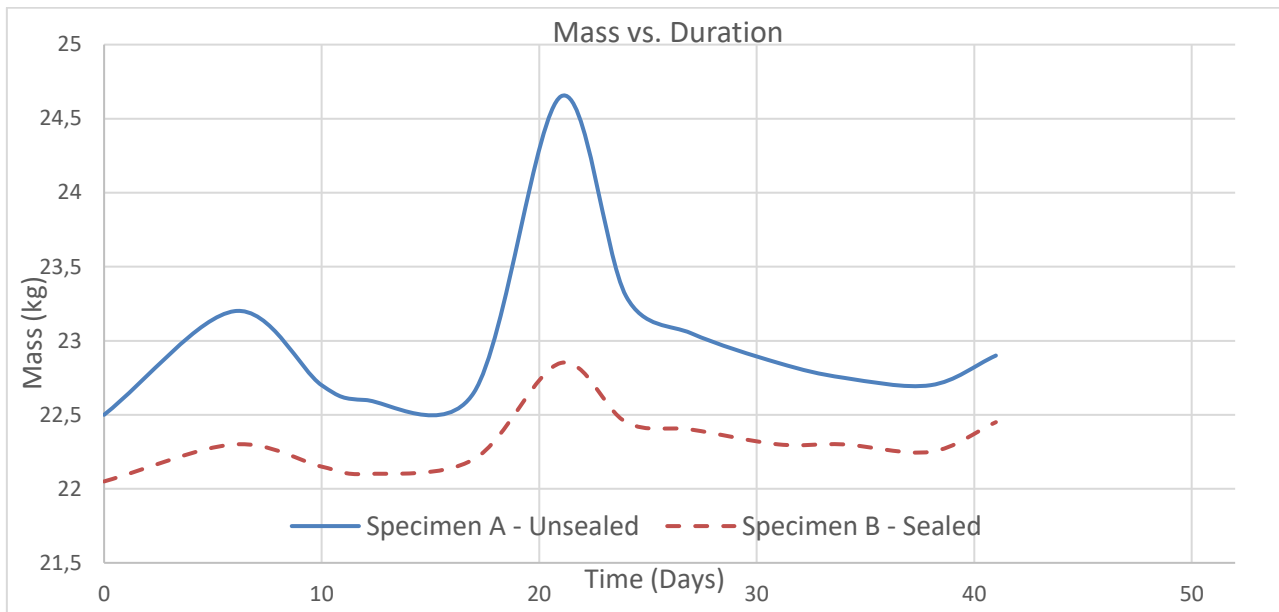
Figure 4: Mass of specimens over the duration of the first 41 days
